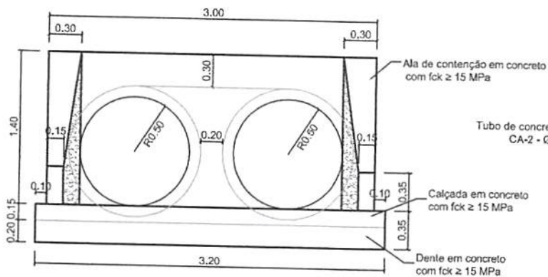
VISTA FRONTAL
